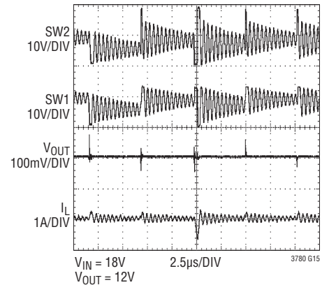
Skip-Cycle Mode ( V_{IN} = 18\text{V} , V_{OUT} = 12\text{V} )
